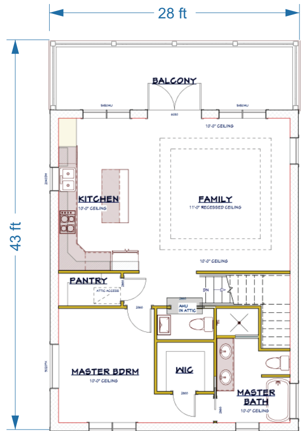
2nd Floor
