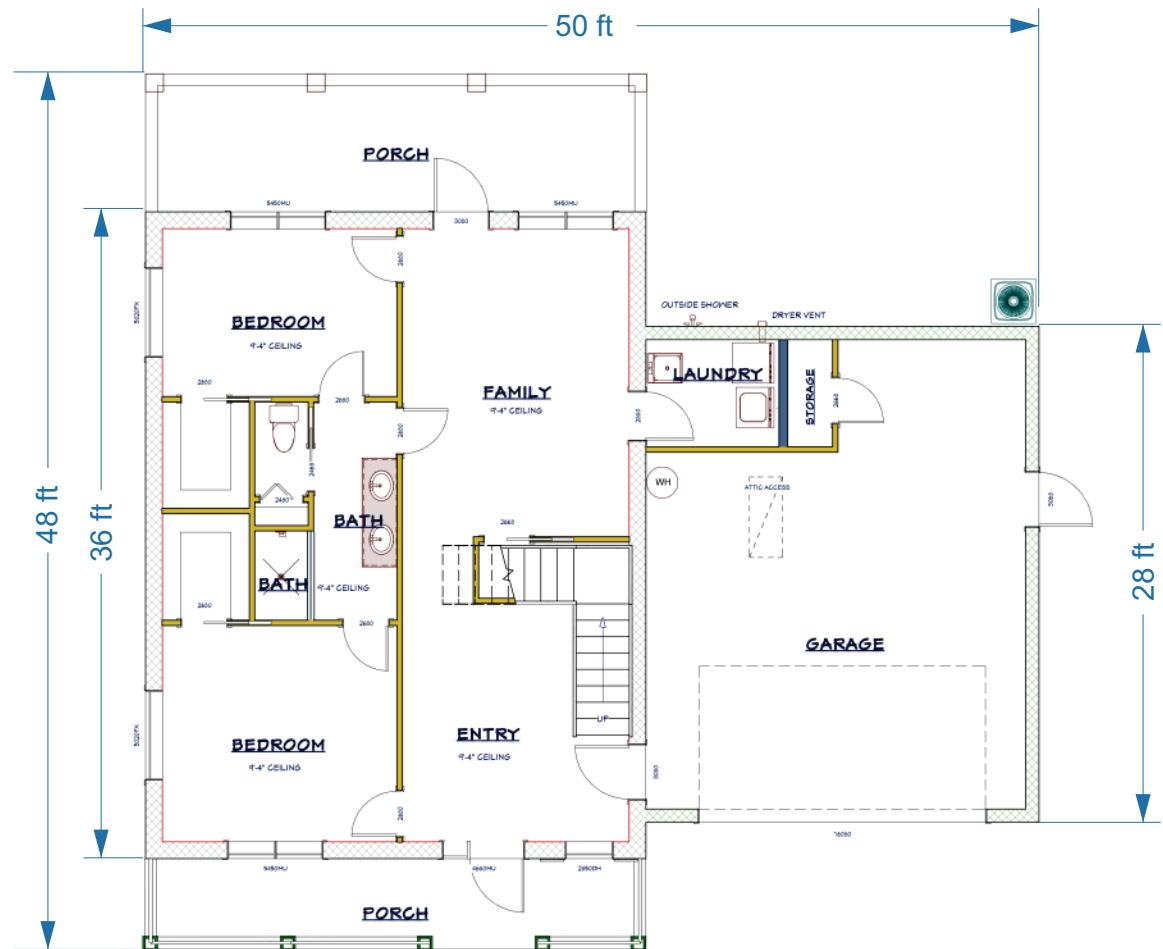
1st Floor
